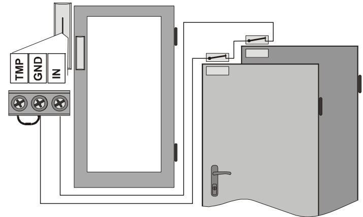
Wiring example
