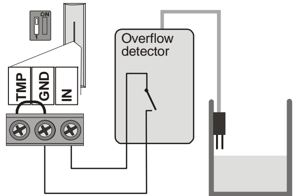
Example of NO contact wiring
